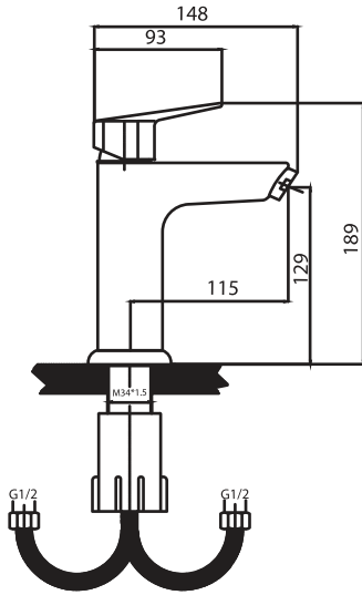
Single lever basin mixer
