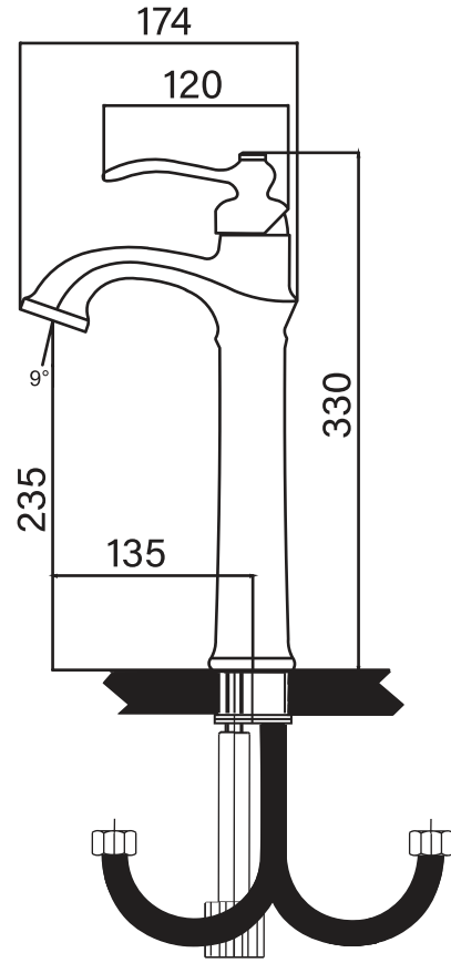
Single lever basin mixer tall
