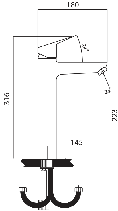
Single lever basin mixer tall
