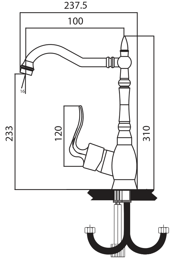
Sink faucet
