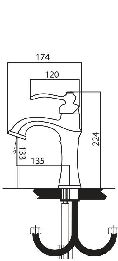
Single lever basin mixer
