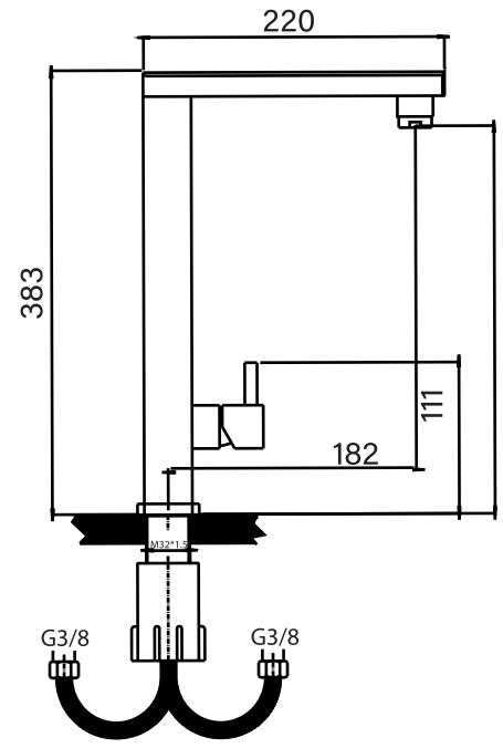
Sink faucet
