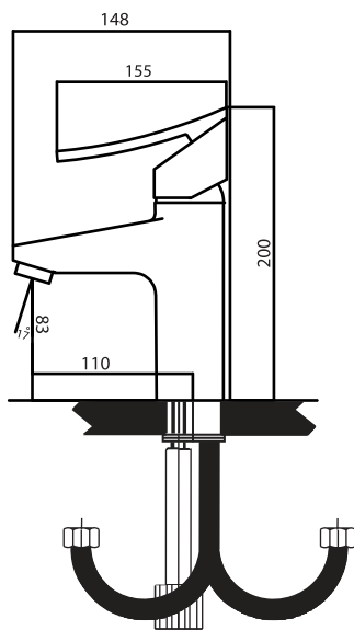
Single lever basin mixer
