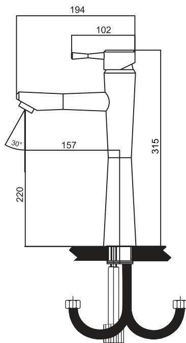
Single lever basin mixer tall
