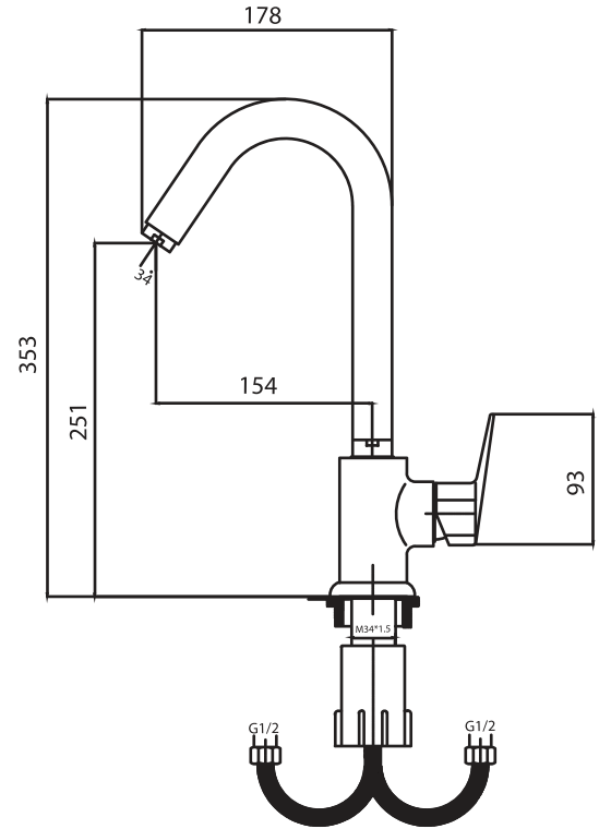
Sink faucet
