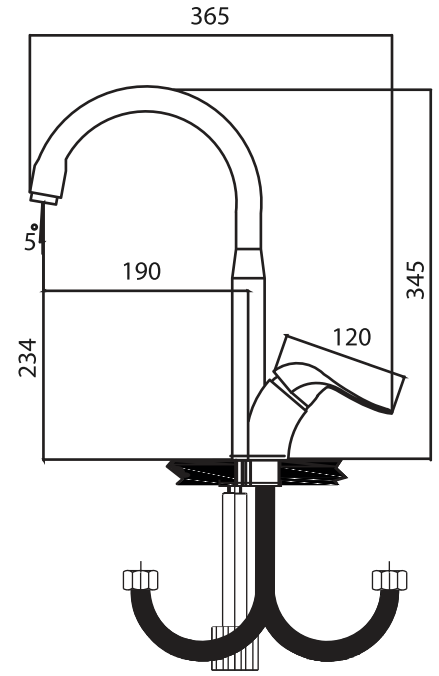
Sink faucet
