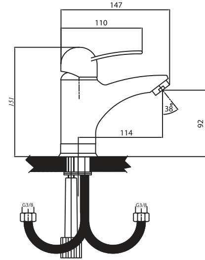
Single lever basin mixer
