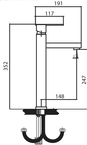
Single lever basin mixer tall
