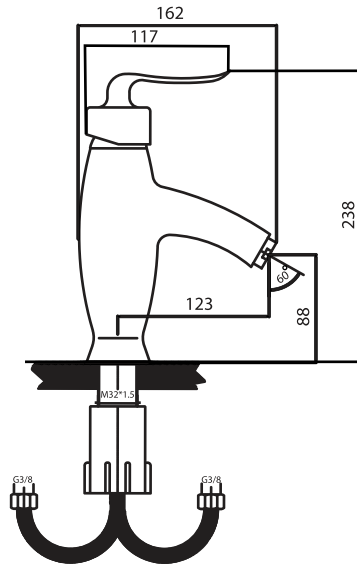
Single lever basin mixer
