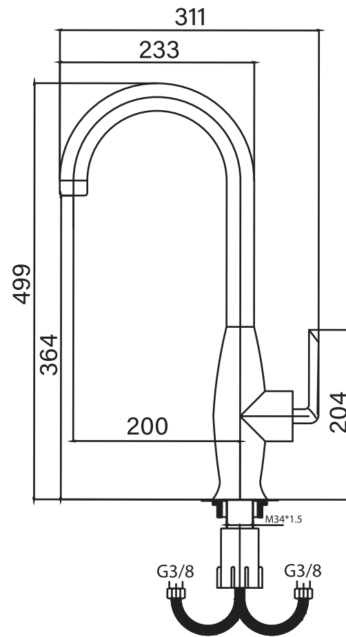
Sink faucet
