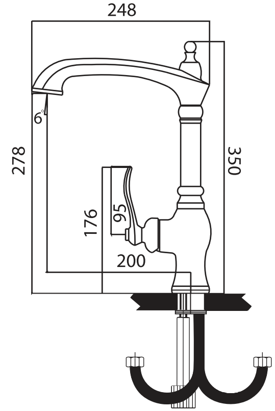
Sink faucet
