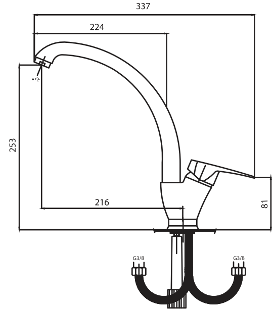
Sink faucet
