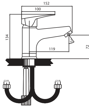
Single lever basin mixer
