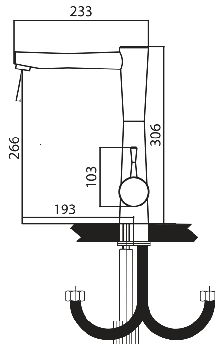
Sink faucet
