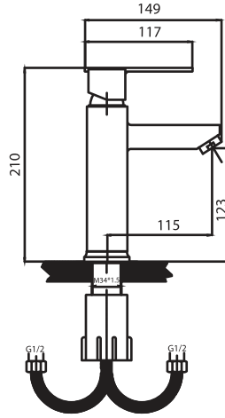
Single lever basin mixer
