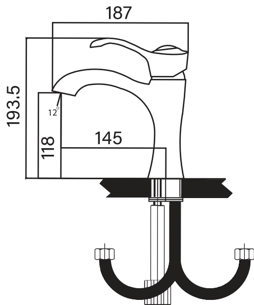
Single lever basin mixer
