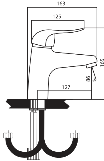
Single lever basin mixer
